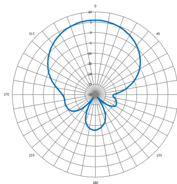
Horizontal (FCC)
