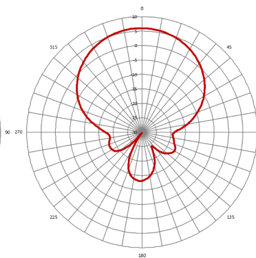
Vertical (FCC)
