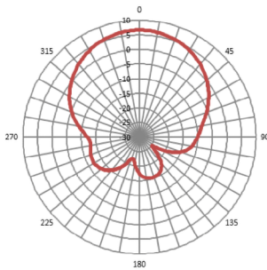
Vertical (FCC)
